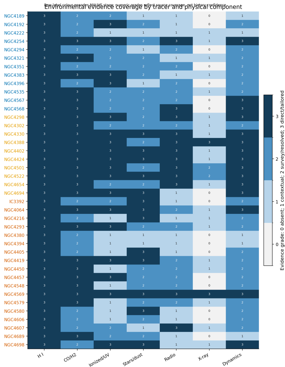
Figure 5. Evidence coverage by tracer. Grade and final-history confidence are deliberately separate.
