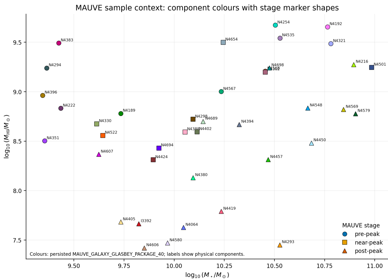
Figure 2. Stellar-mass–H I-mass context for the same physical components.
