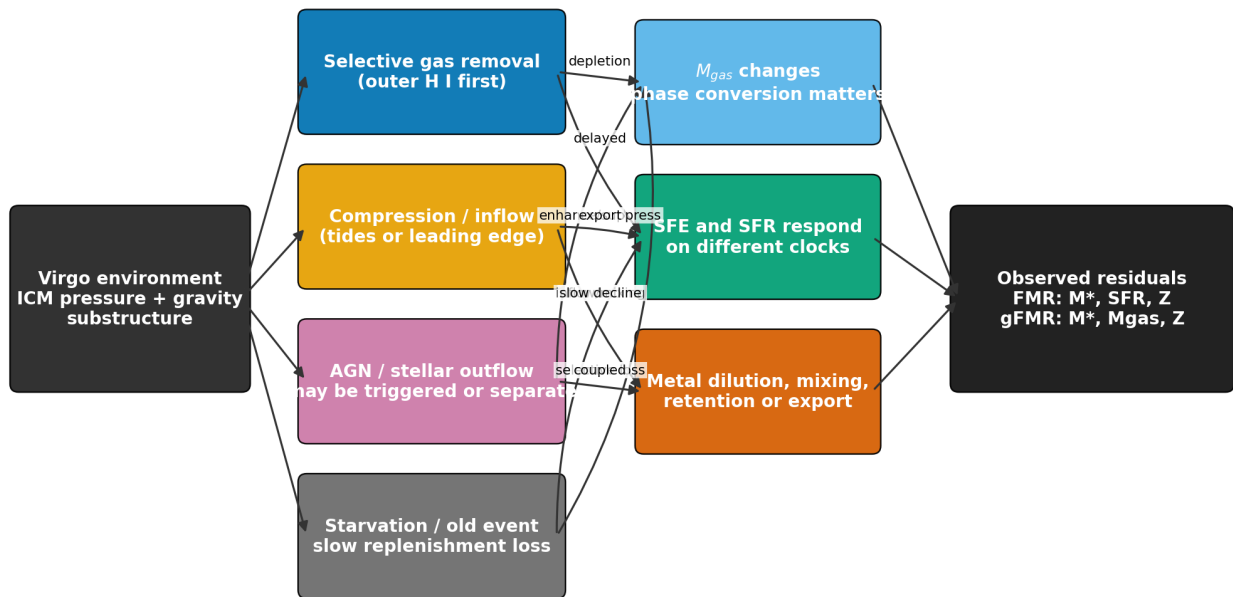
Figure 8. Environmental pathways through FMR/gFMR observable space; a population relation is not an evolutionary track.
