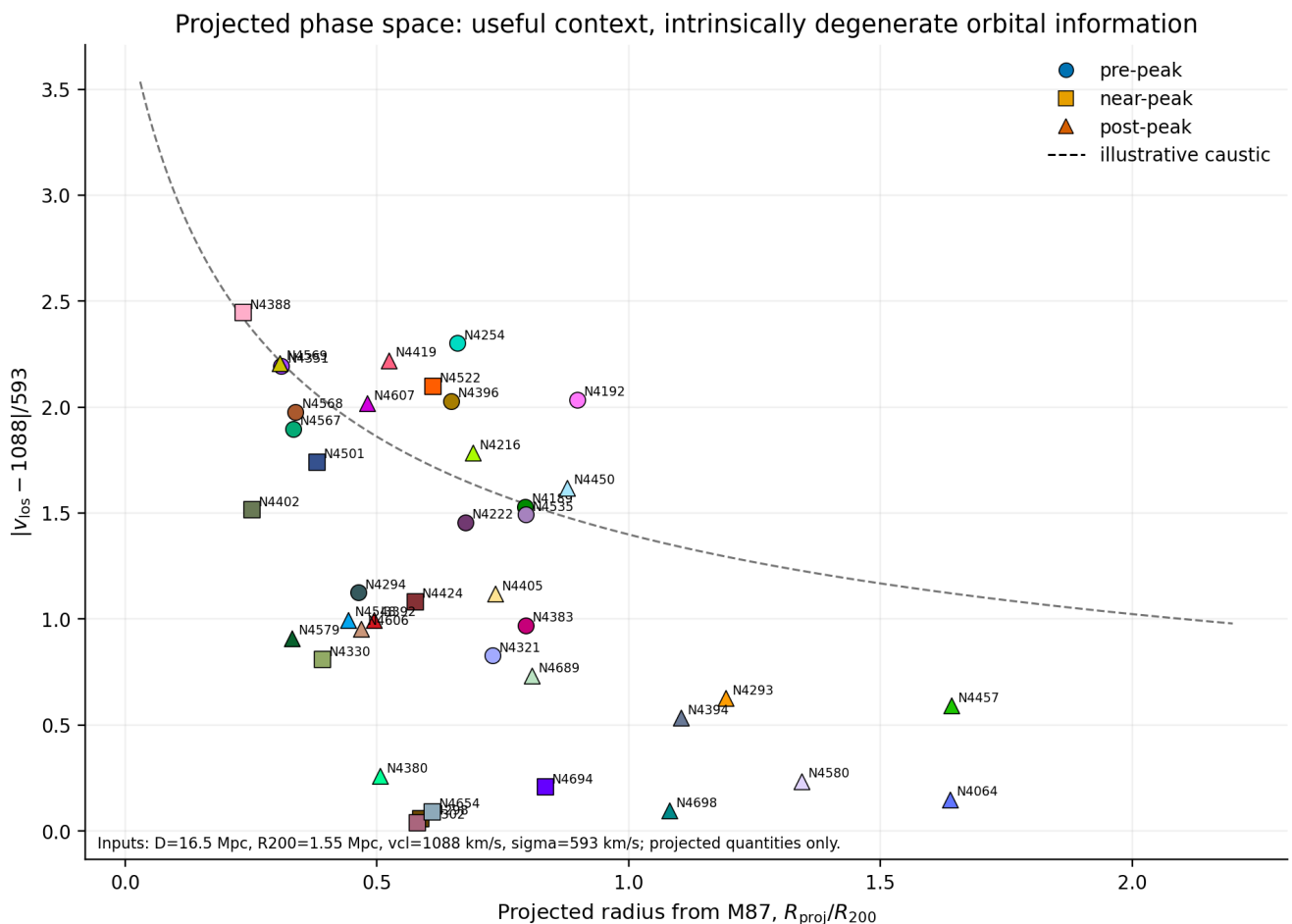
Figure 3. Projected phase space. This is statistical context, not a unique reconstruction of any orbit.
