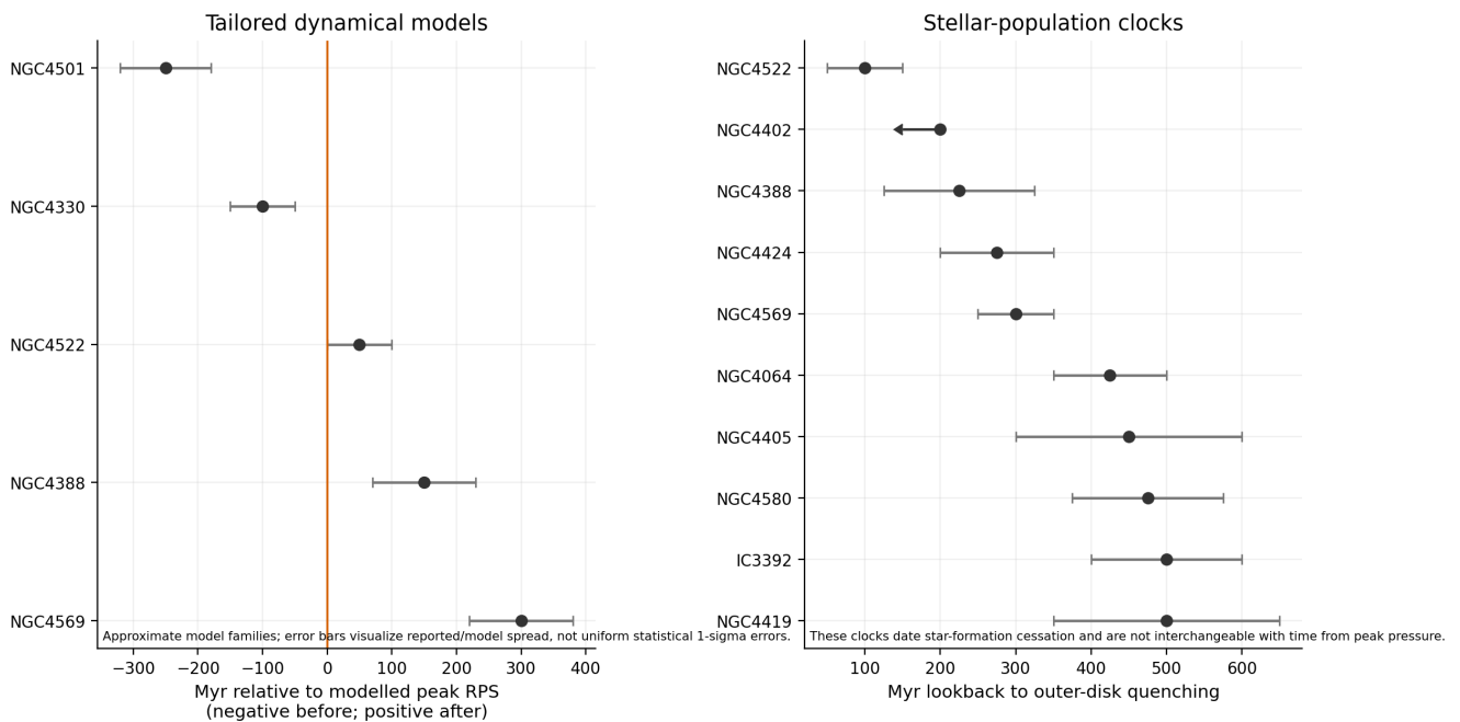
Figure 7. Published dynamical and stellar-population clocks, shown in separate panels because they date different physical events.
